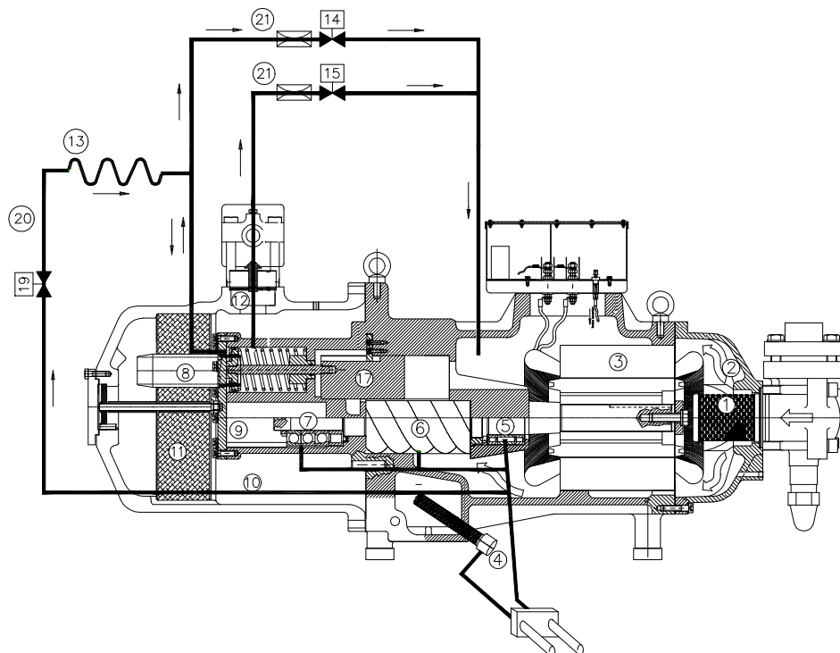
oil circuit layout in the LZ configuration;
