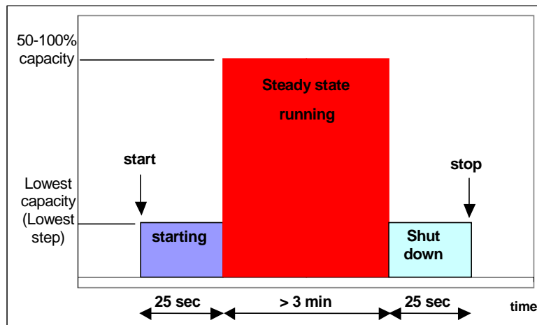
Picture 3-Z: starting and stopping the compressor;
